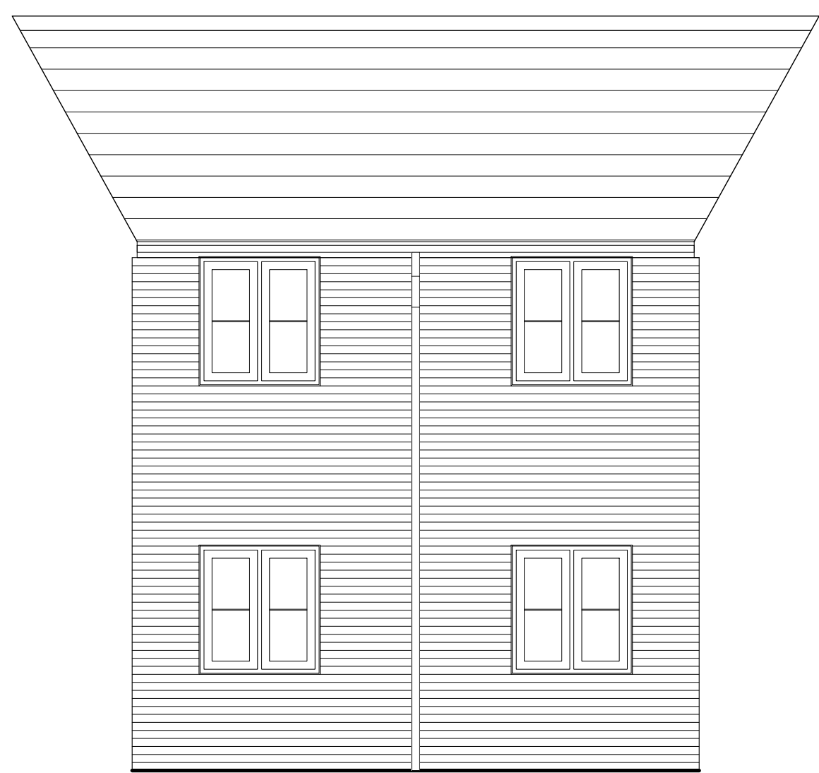
Rear elevation
