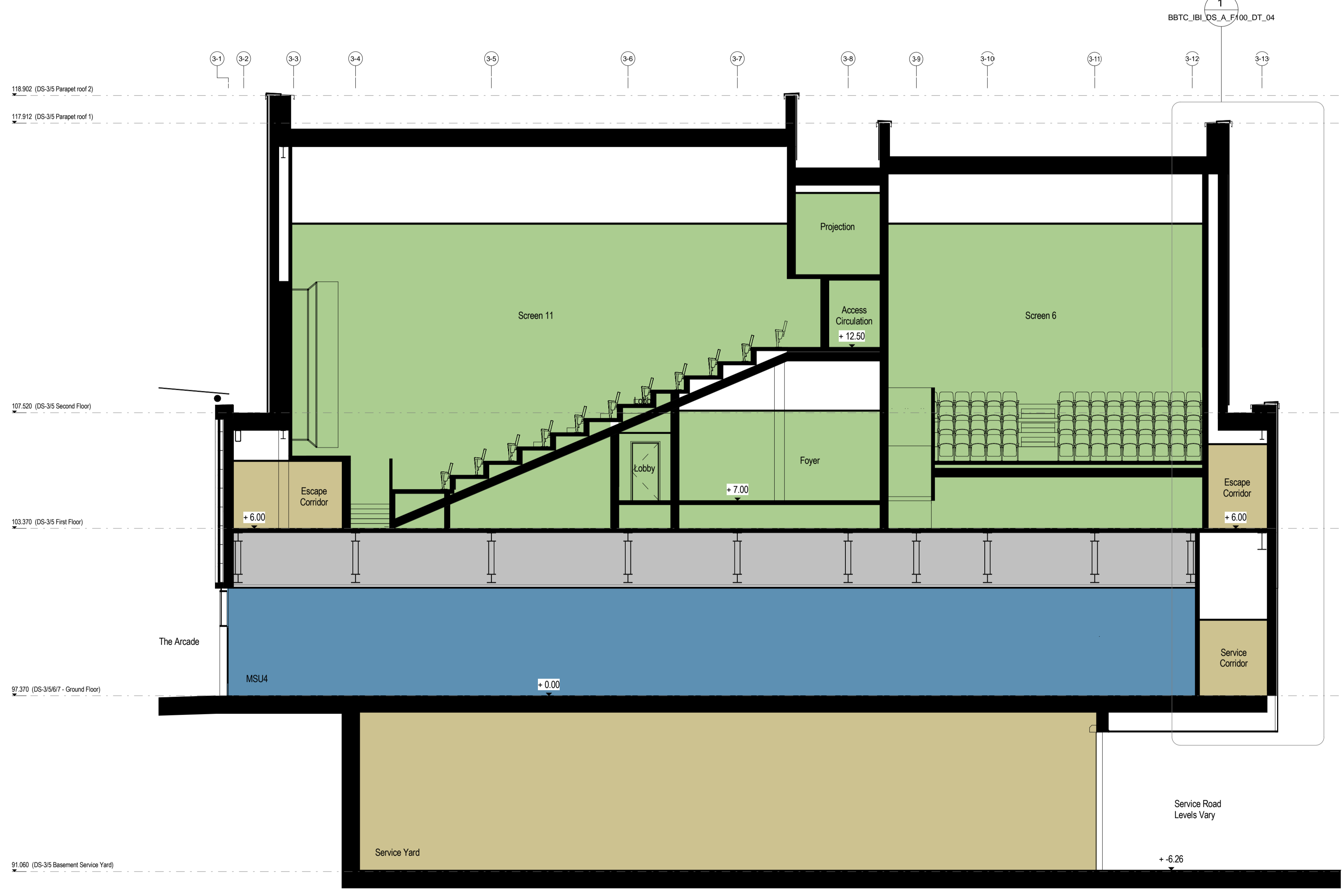
B Section B 1:100
