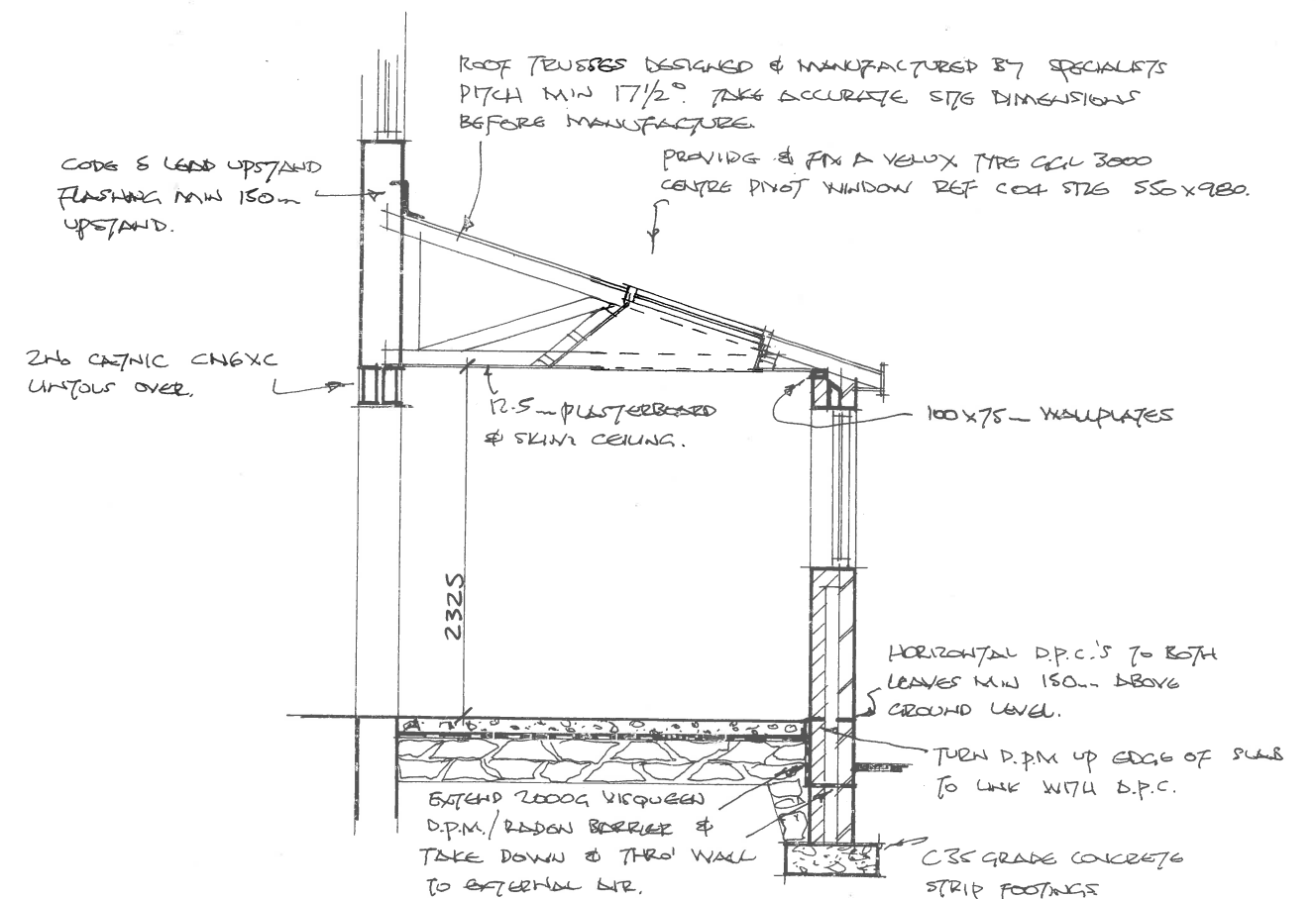
SECTION A-A (1:50)
