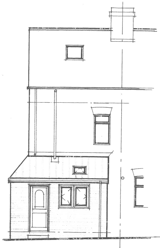
PROP. REAR ELEVATION (1:100)
