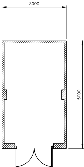
PROPOSED PLAN SCALE 1:100 AT A3
