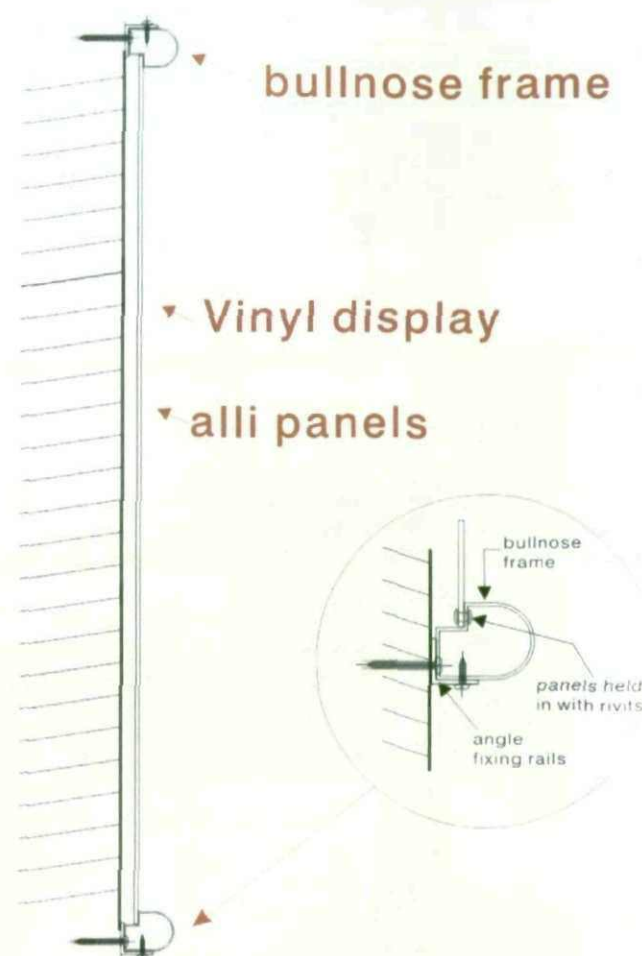
SIGN A- scale 1:5
