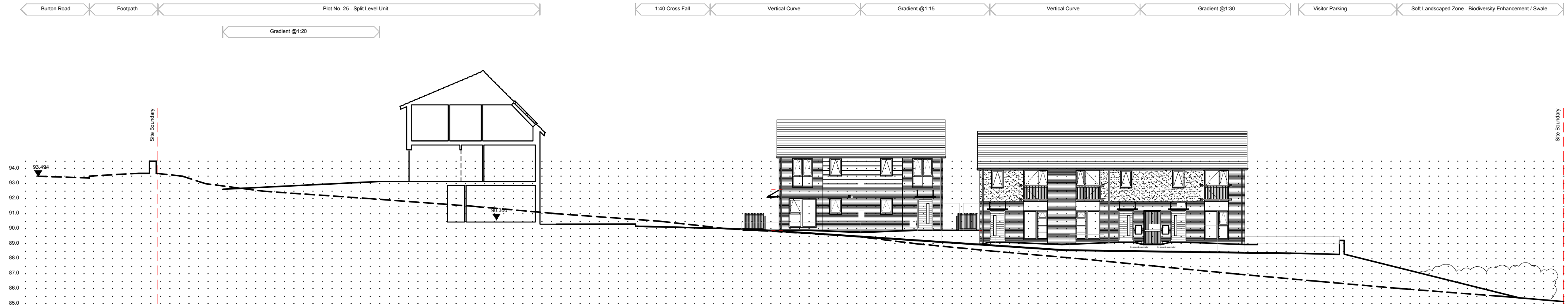
Section 3
