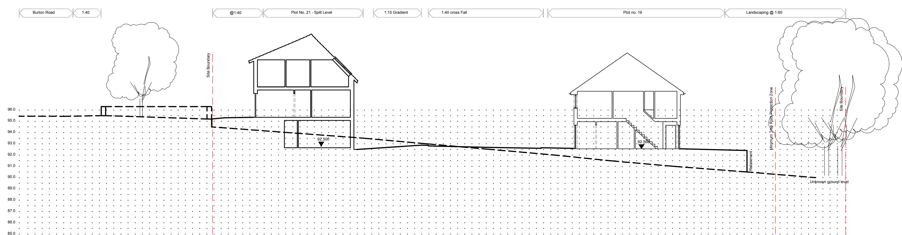
Section 4
