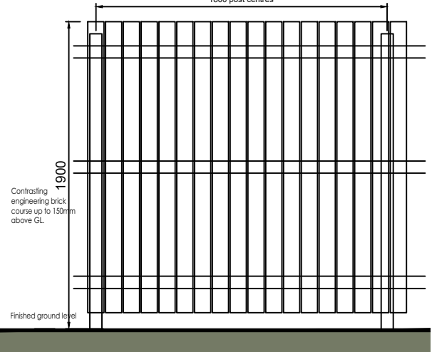
1.8m Boundary screen fence
