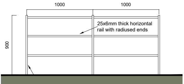
0.9m Estate railings
