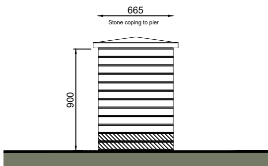
Brick pillar detail
