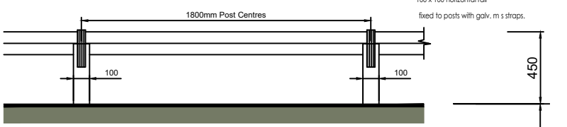
0.45m Knee railing
