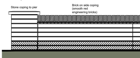
0.6m Low frontage wall
