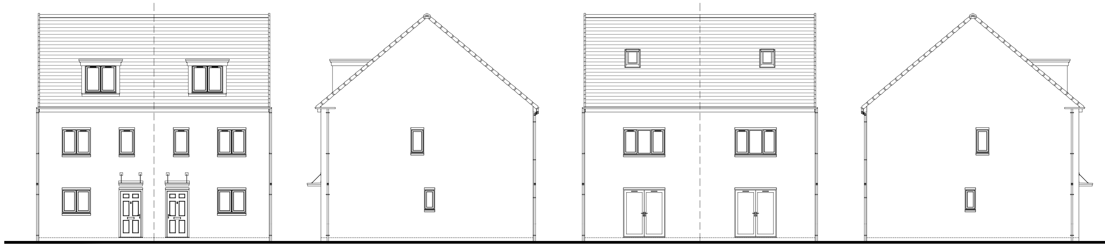
FRONT ELEVATION
