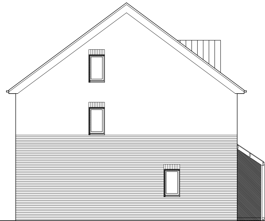
Side Elevation Plot 6
