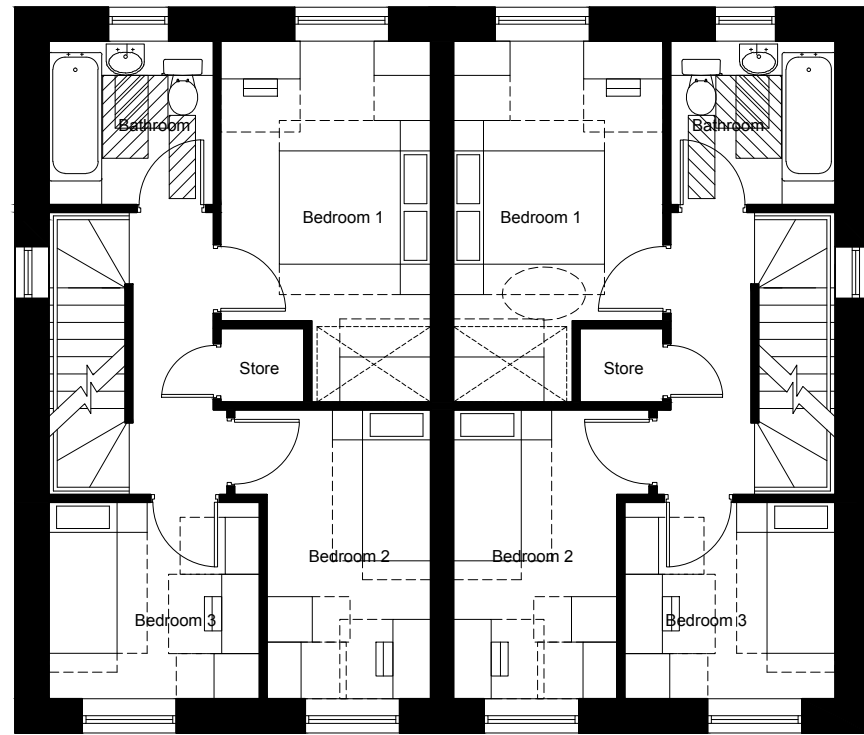
4B6P - Plot 6 4B6P - Plot 5 First Floor
