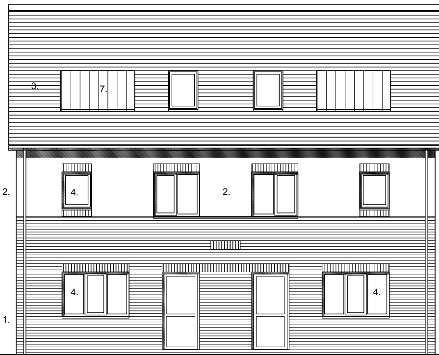
Rear Elevation Plots 5 & 6
