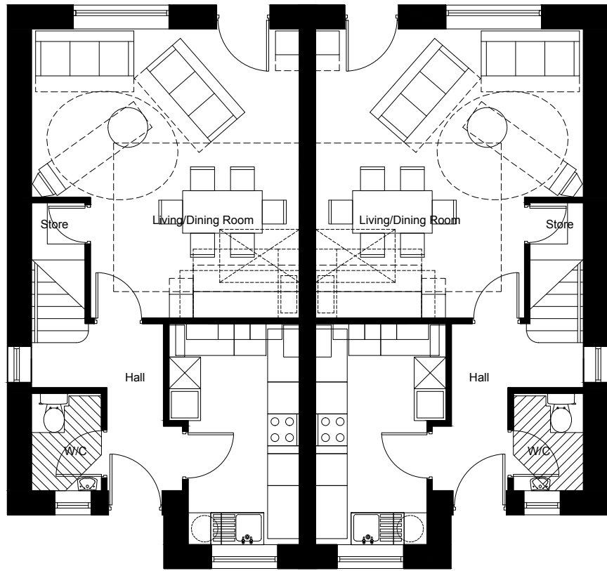
4B6P - Plot 6 4B6P - Plot 5 Ground Floor Plot size - 116 m²
