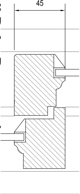
Detail D As Proposed
