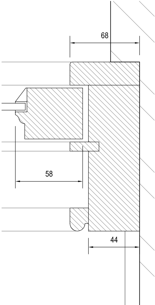
Detail C As Proposed
