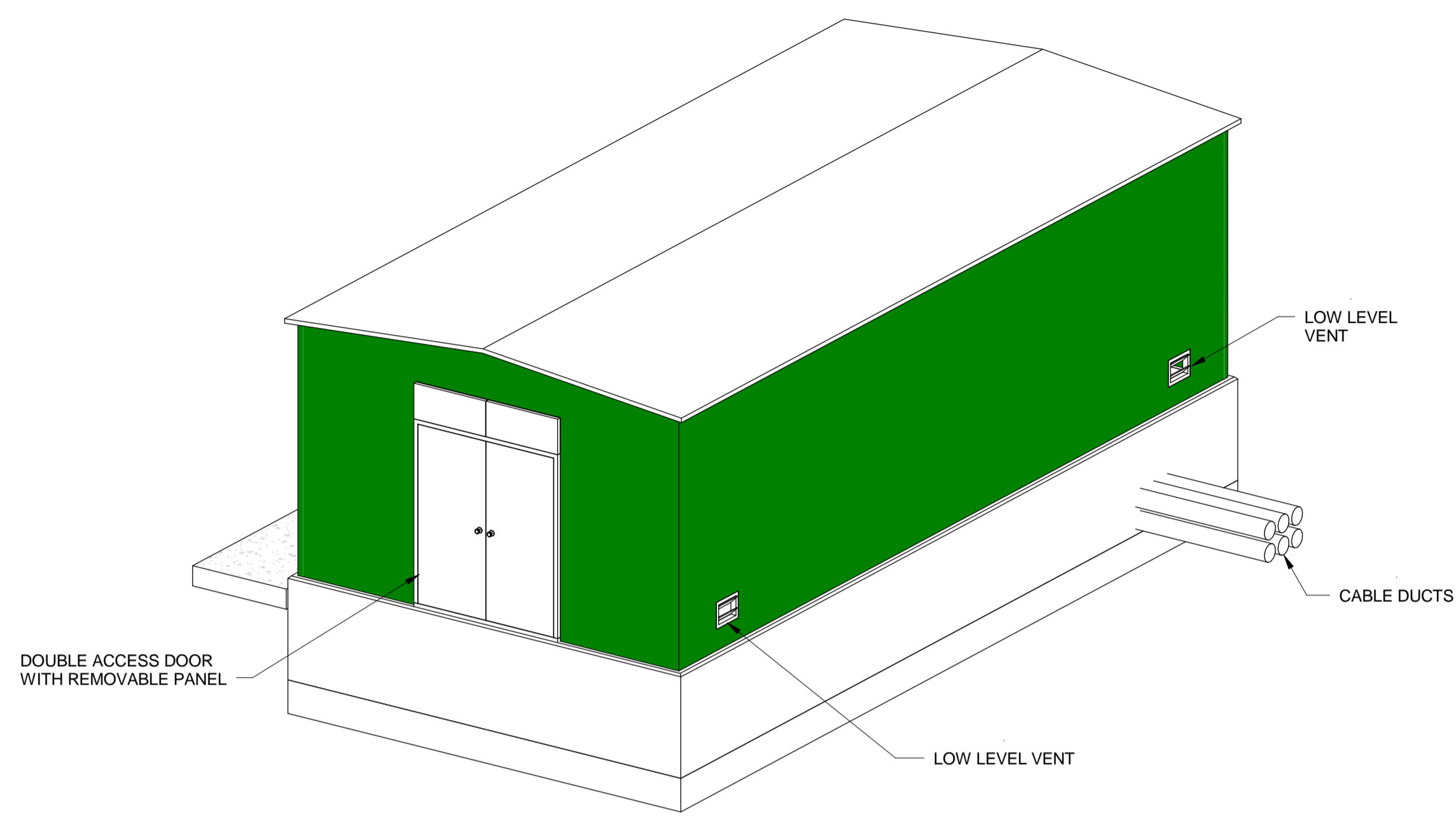
6 3D VIEW MCC BUILDING
