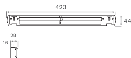
Acoustic spacer
