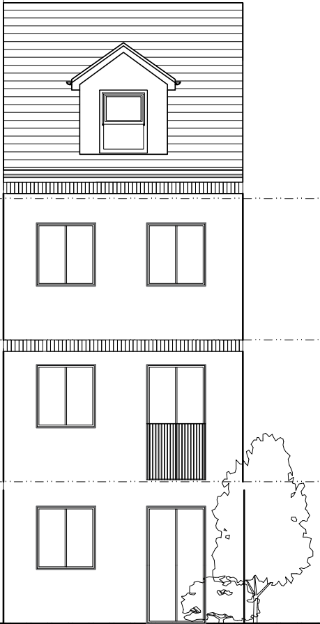
REAR ELEVATION
