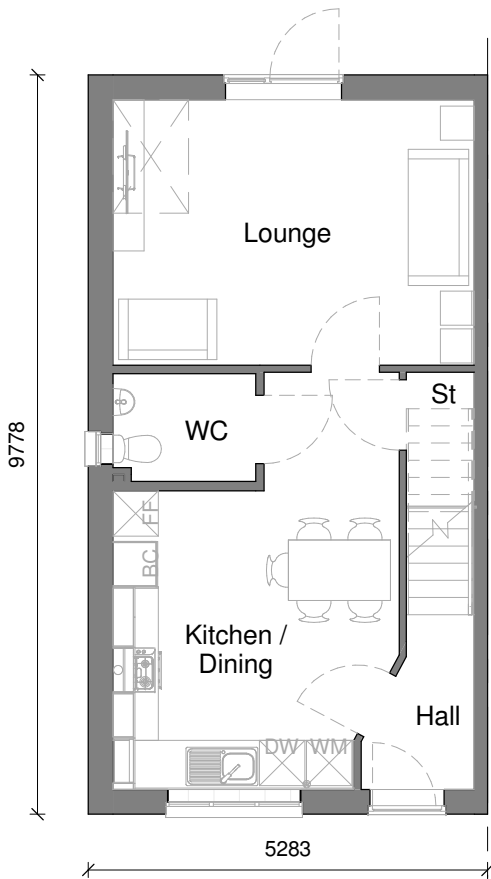
Ground Floor. 1 : 100
