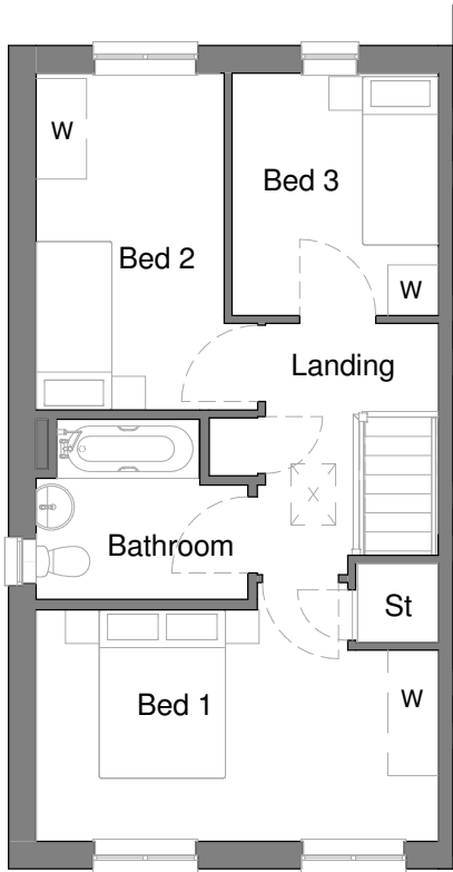
First Floor. 1 : 100
