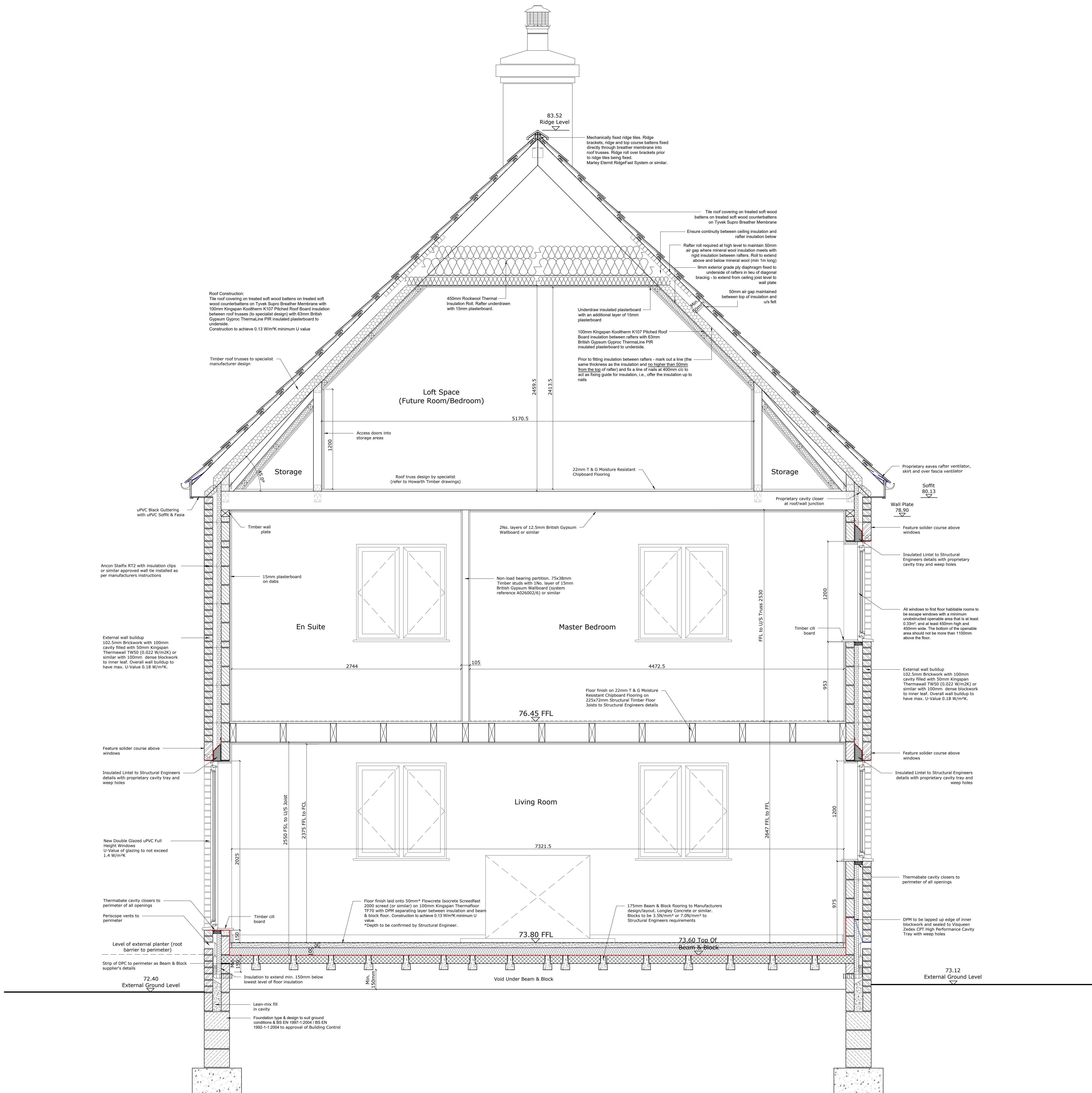
SECTION B-B
