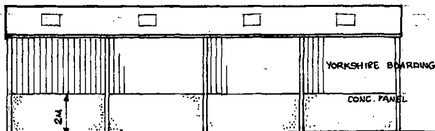
REAR
