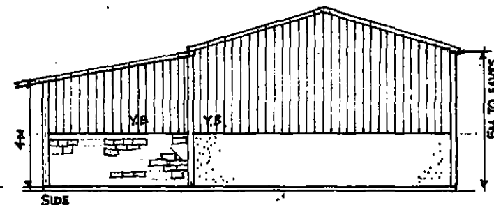
SHEEP SHELTER BARN. DRG A1. 2022 SCALE 1:200
