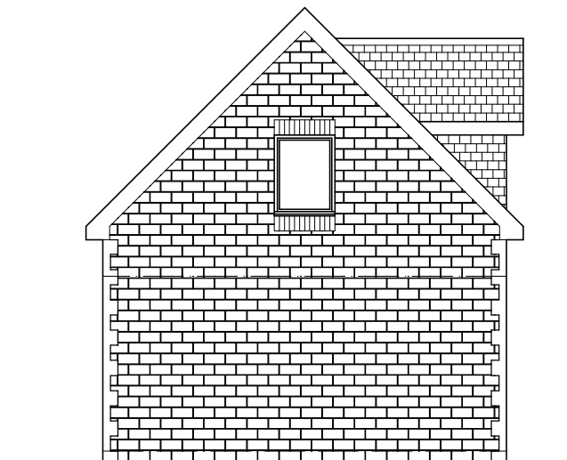
SIDE ELEVATION
