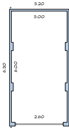
Single Garage Plan
