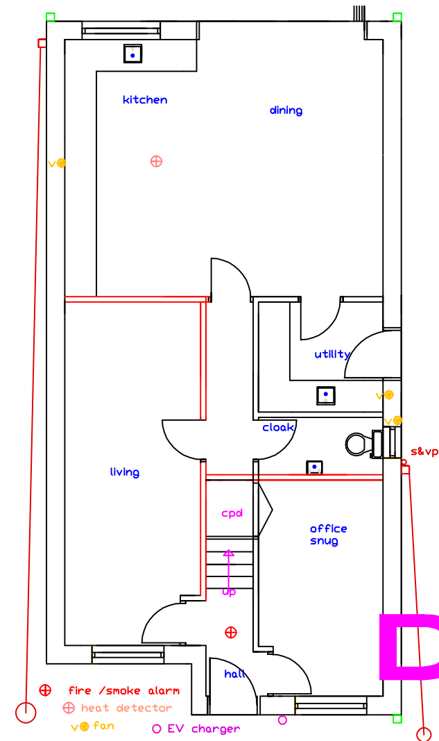
PROPOSED GROUND FLOOR LAYOUT 1:100
