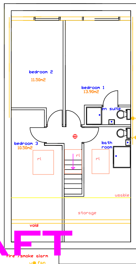
PROPOSED FIRST LOFT FLOOR LAYOUT 1:100
