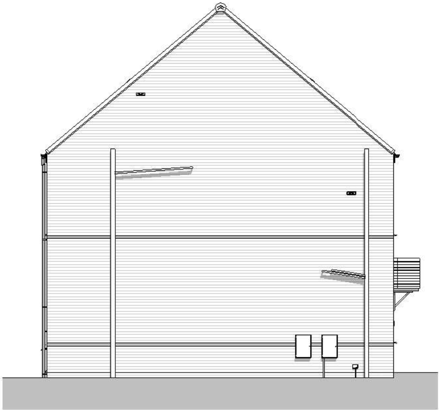
Left Elevation 1 : 100
