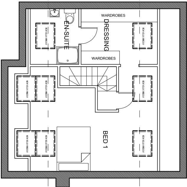
PROPOSED SECOND FLOOR PLAN SCALE 1:100
