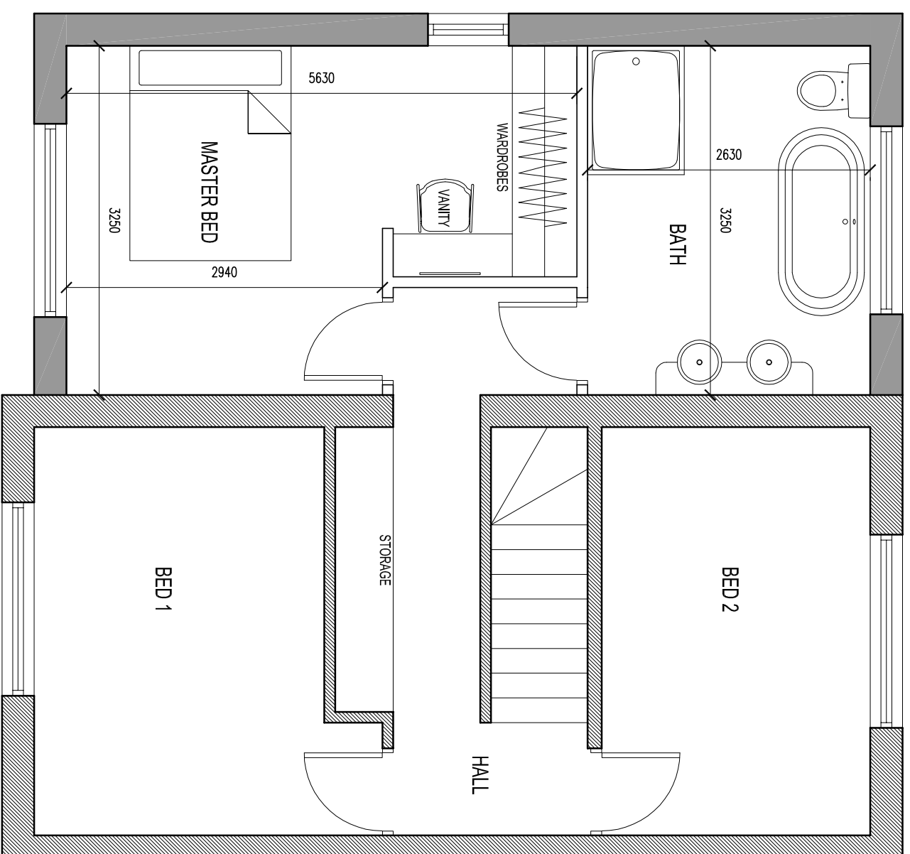
PROPOSED FIRST FLOOR PLAN SCALE 1:50
