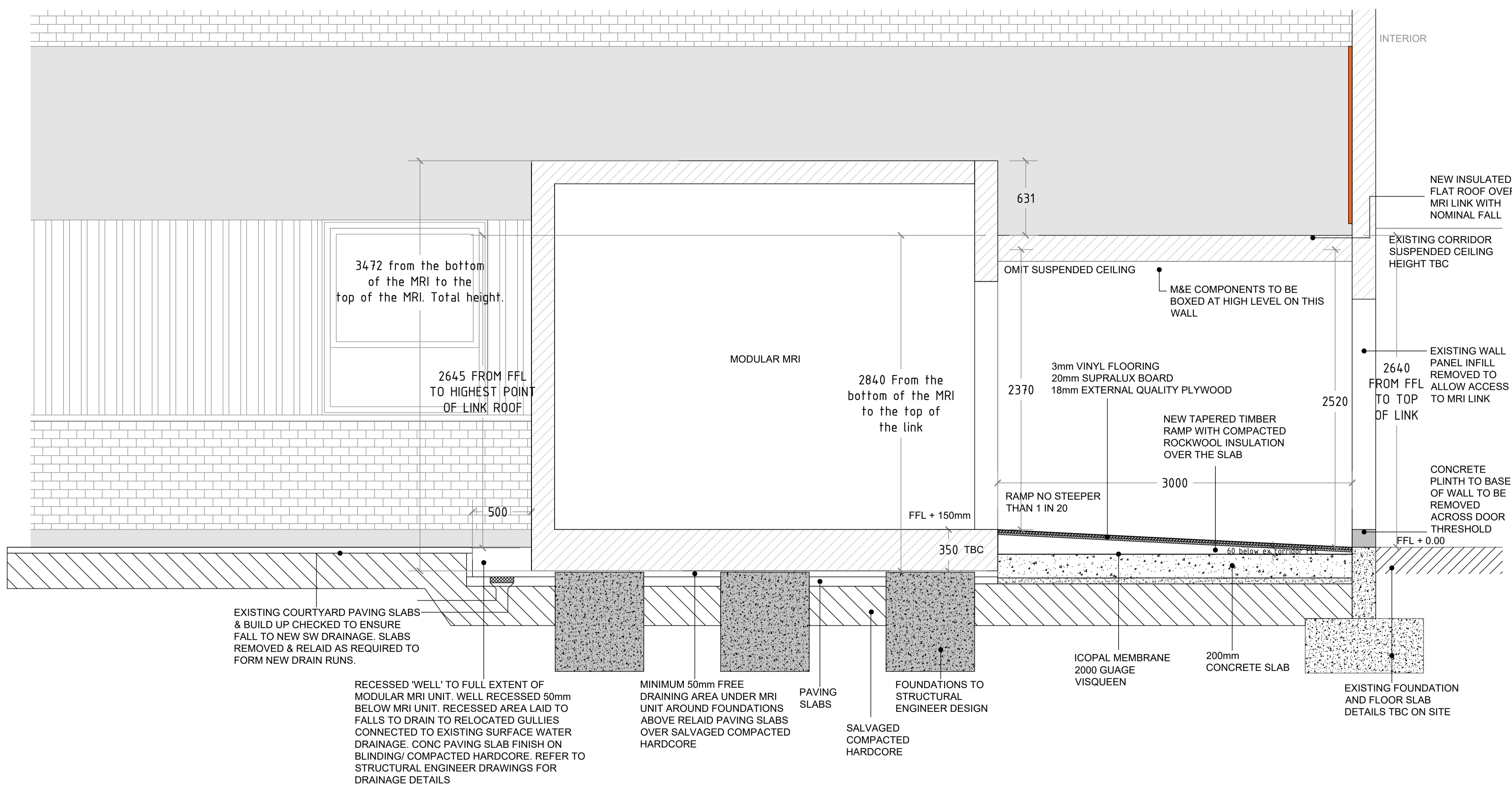
PROPOSED SECTION A 1:20
