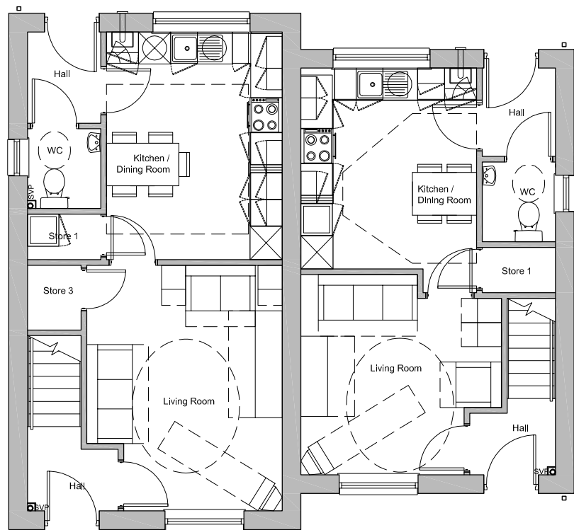
Ground Floor 3B5P Type B - Plot 1 or 8 2B4P Type A - Plot 2 or 9
