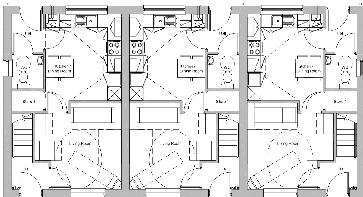
Ground Floor 2B4P Type A - Plot 3 2B4P Type A - Plot 4 2B4P Type A - Plot 5
