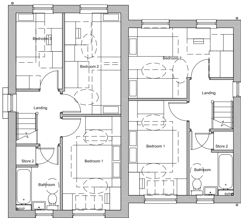
First Floor 3B5P Type B - Plot 1 or 8 2B4P Type A - Plot 2 or 9
