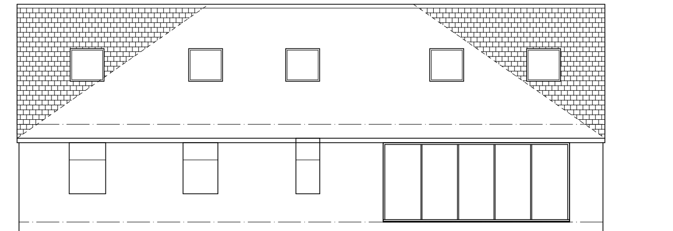
REAR ELEVATION
