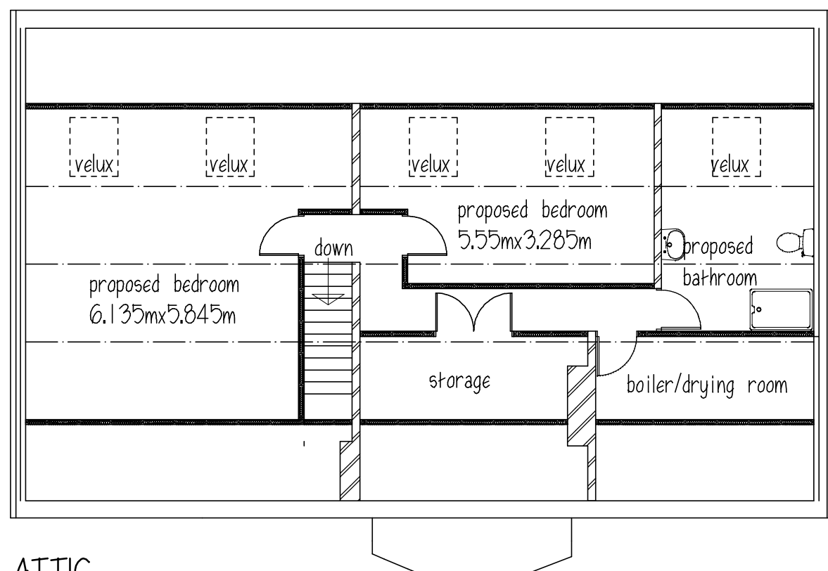
ATTIC
