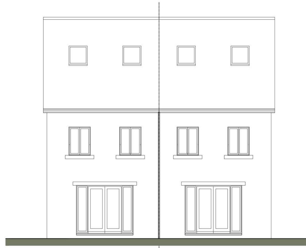
REAR ELEVATION
