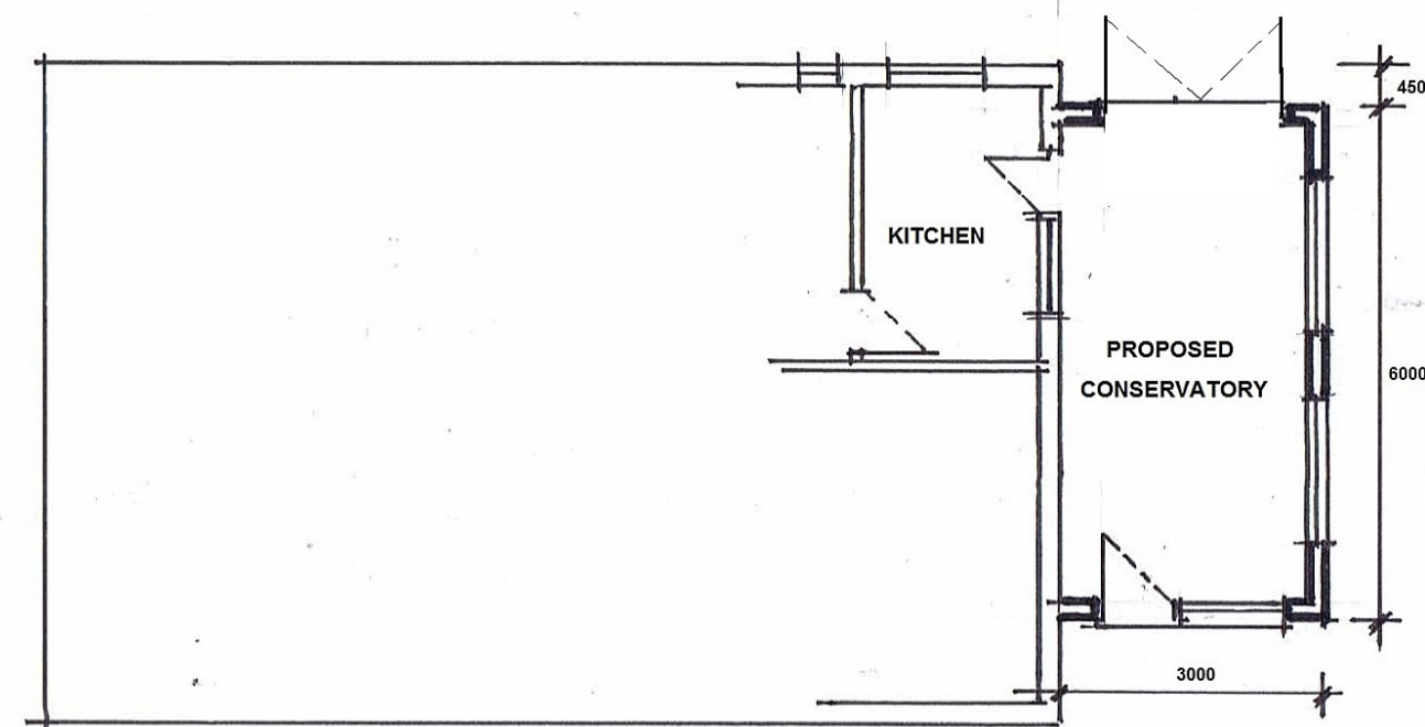
PROPOSED PLAN
