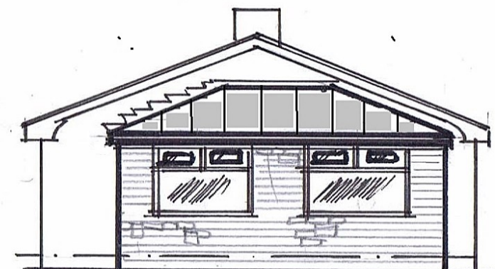
PROPOSED RIGHT SIDE ELEVATION
