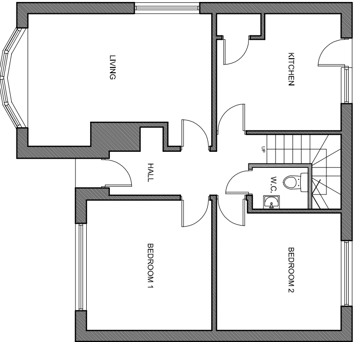
PROPOSED GROUND FLOOR PLAN SCALE 1:100
