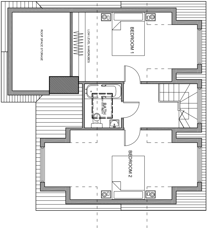
PROPOSED FIRST FLOOR PLAN - OPTION 2 SCALE 1:100
