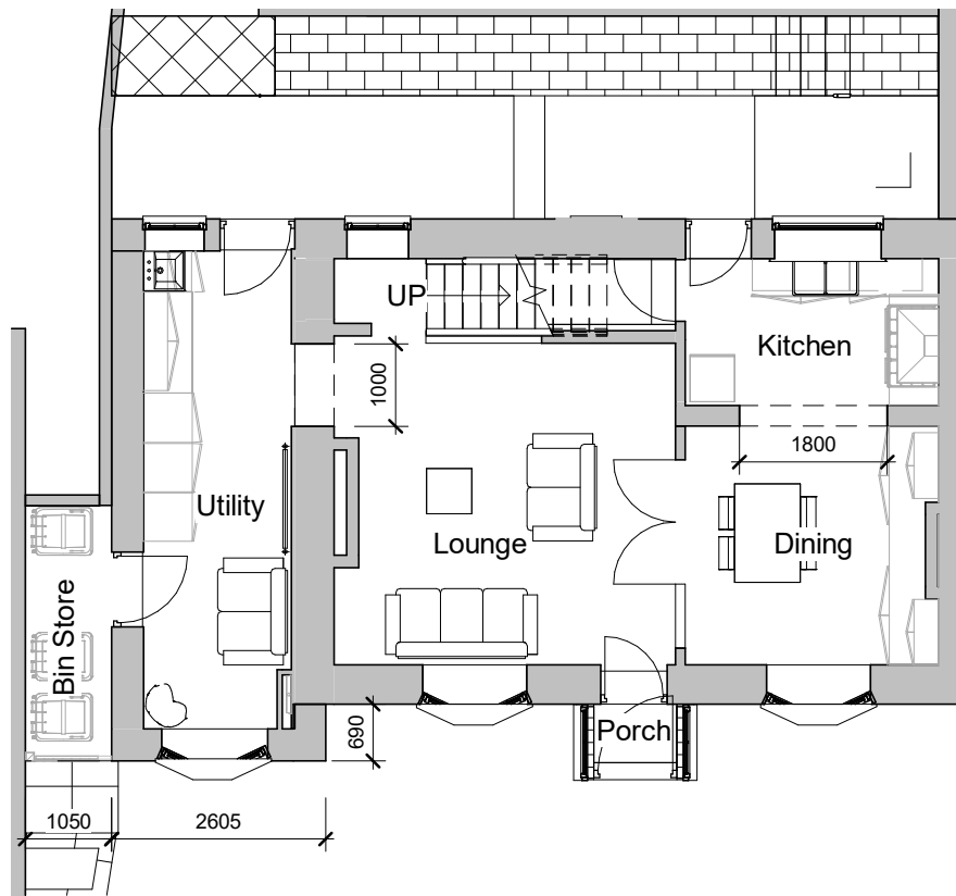
Ground Floor Plan Proposed 1 : 100
