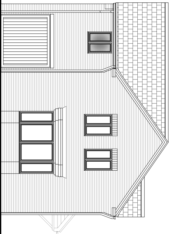
Front/Side Elevation
