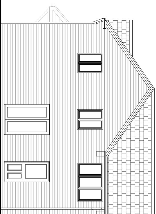
Rear Elevation
