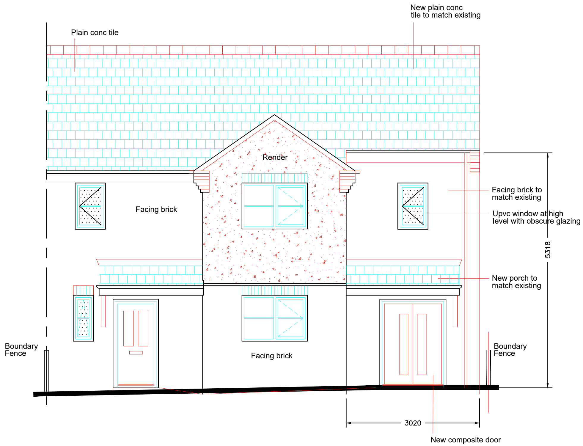
Proposed Front Elevation 1:50
