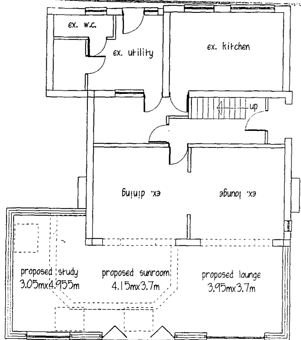
GROUND FLOOR
