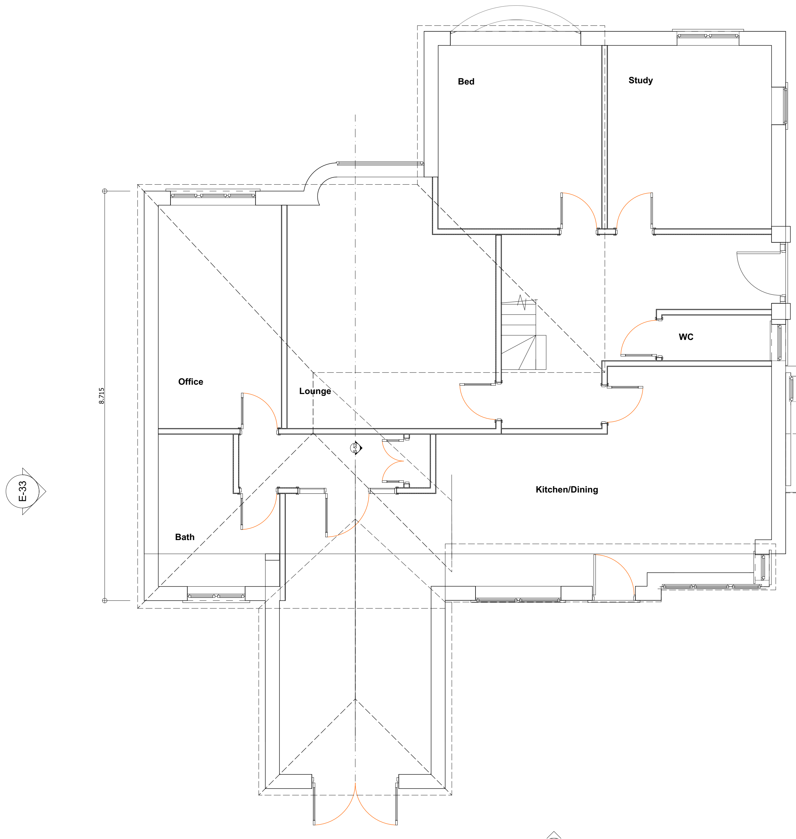
0. Ground Floor (23) 1:50
