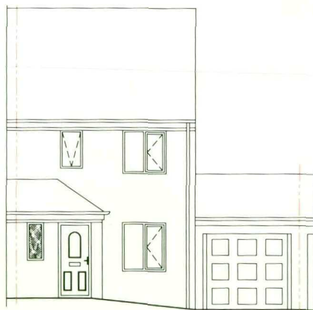
Front Elevation Existing 1:100
