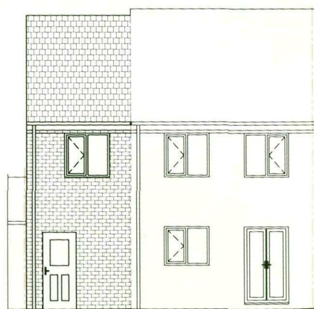
Rear Elevation Proposed 1:100
