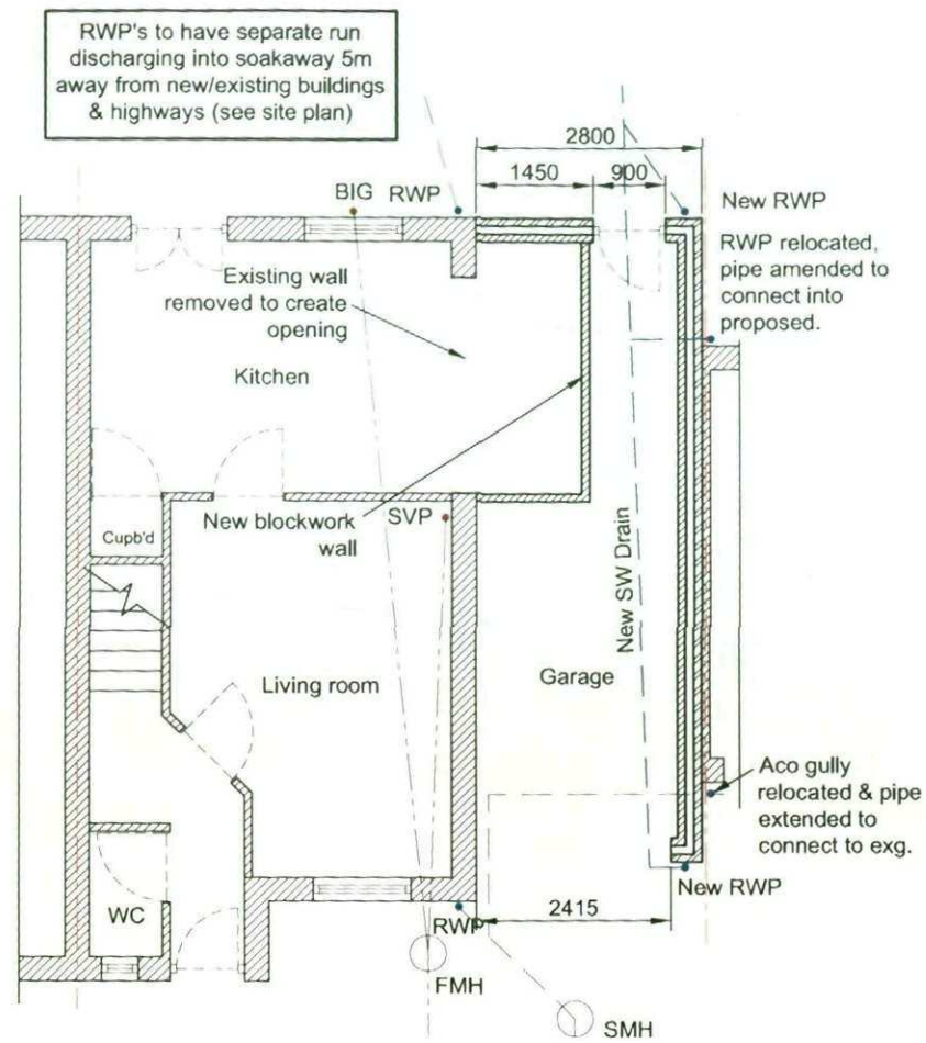
Ground Floor Proposed 1:100
