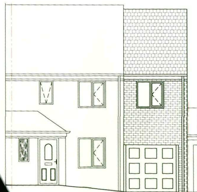
Front Elevation Proposed 1:100
