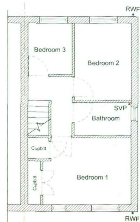
First Floor Existing 1:100
