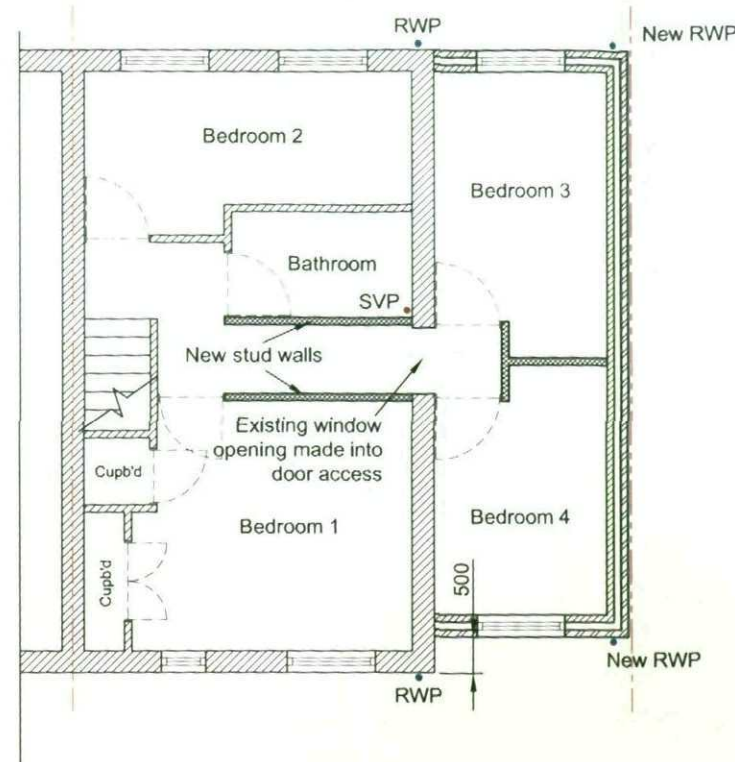
First Floor Proposed 1:100
