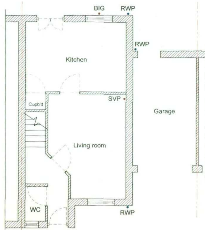
Ground Floor Existing 1:100
