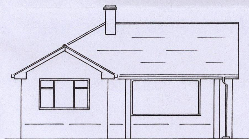
EXISTING FRONT NORTH-EAST
