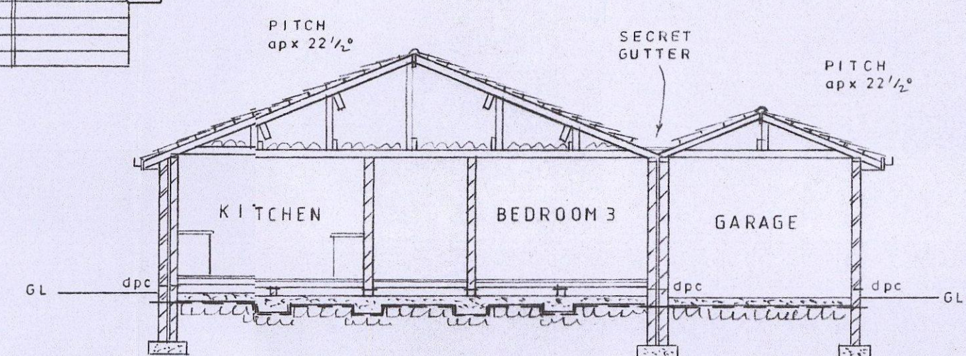
SECTION
