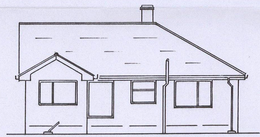
EXISTING REAR SOUTH-WEST
