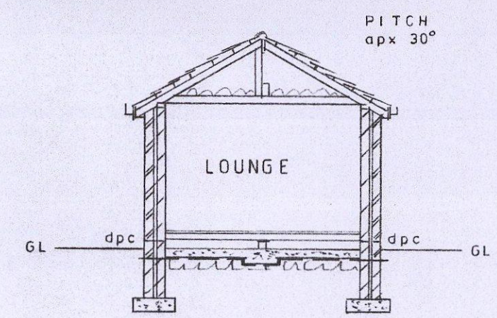
SECTION
