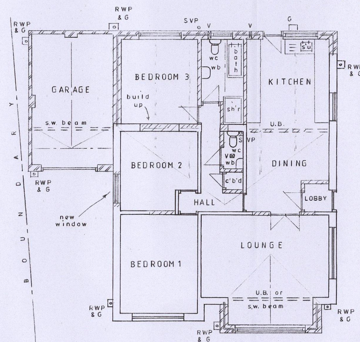
PROPOSED PLAN
