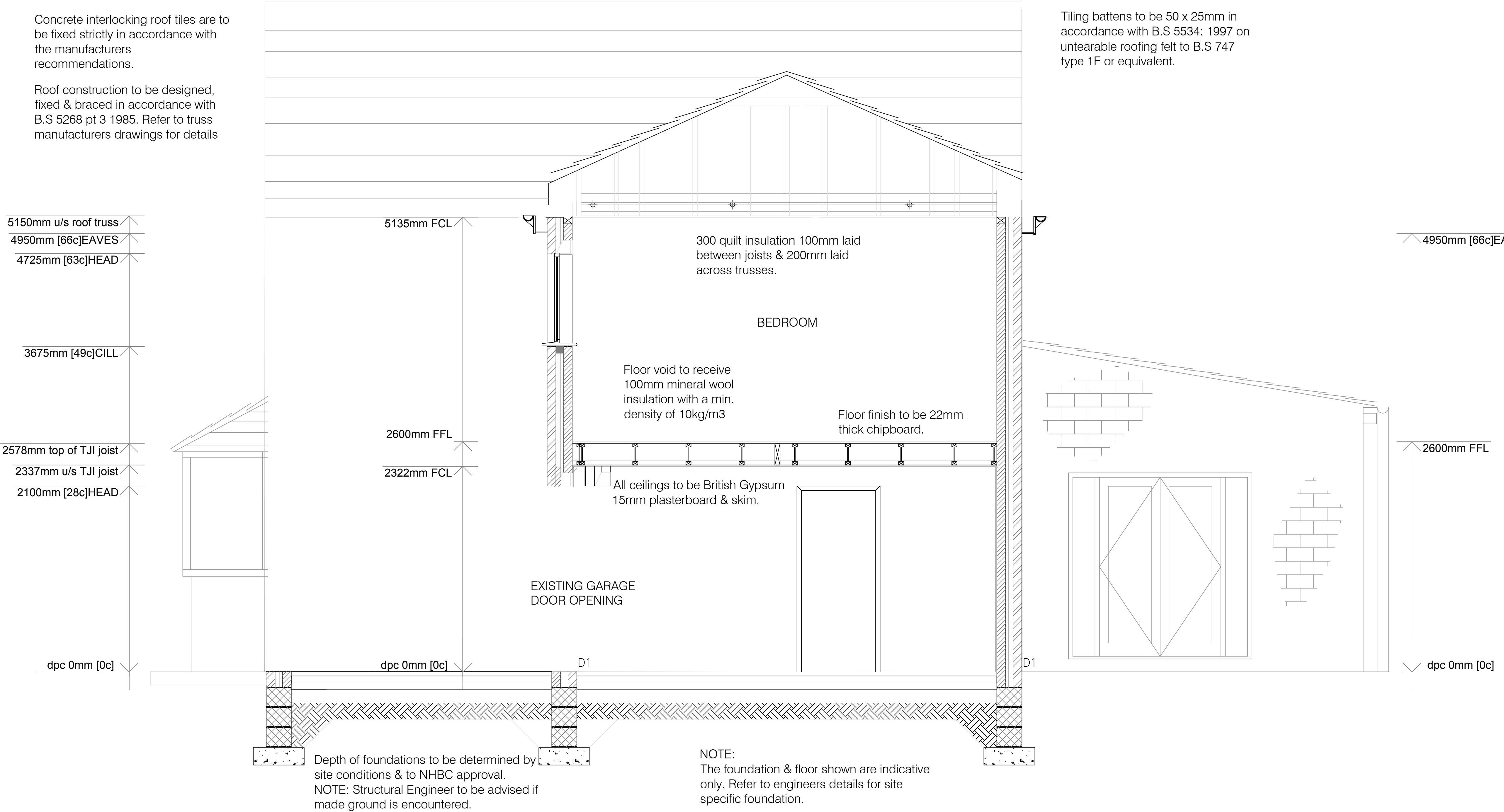
Proposed Section A-A
