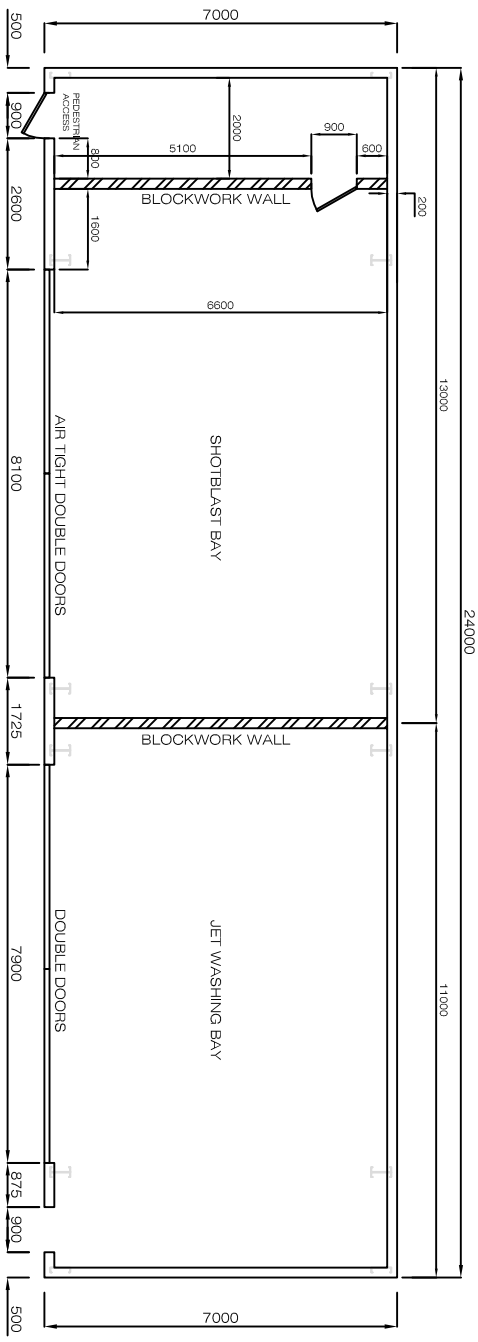
PROPOSED GROUND FLOOR
