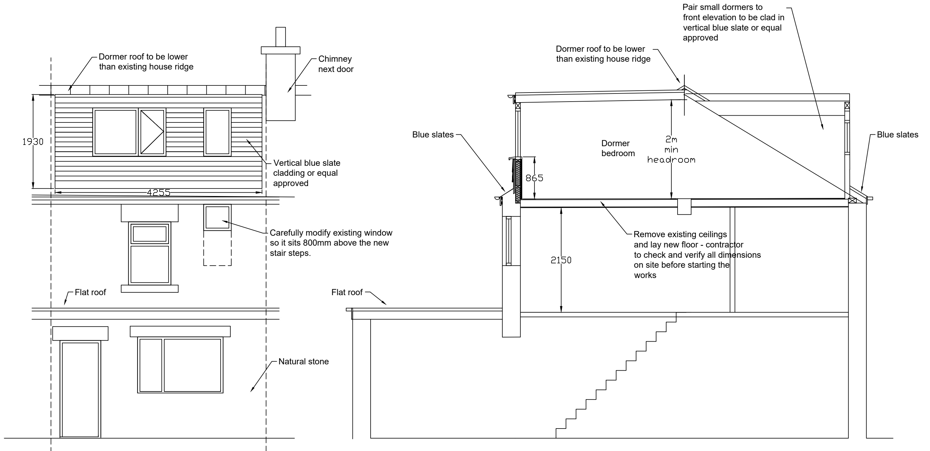
Proposed longitudinal section 1:50
