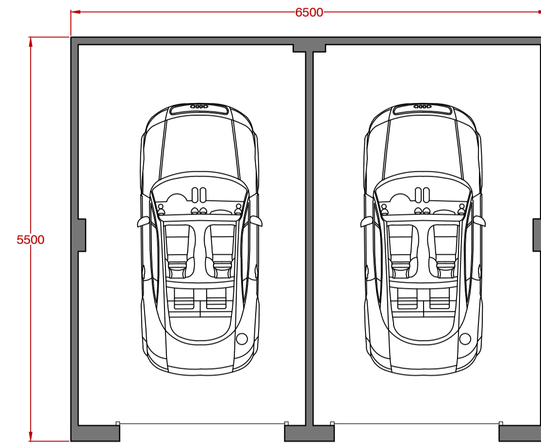
Schematic Floor Plan 1:50
