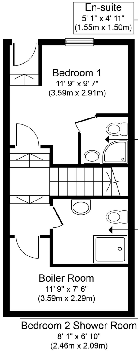
Basement Approximate Floor Area 344 sq. ft. (32.0 sq. m.)
