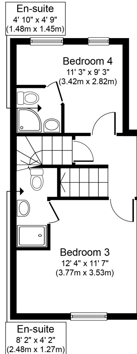
First Floor Approximate Floor Area 323 sq. ft. (30.0 sq. m.)
