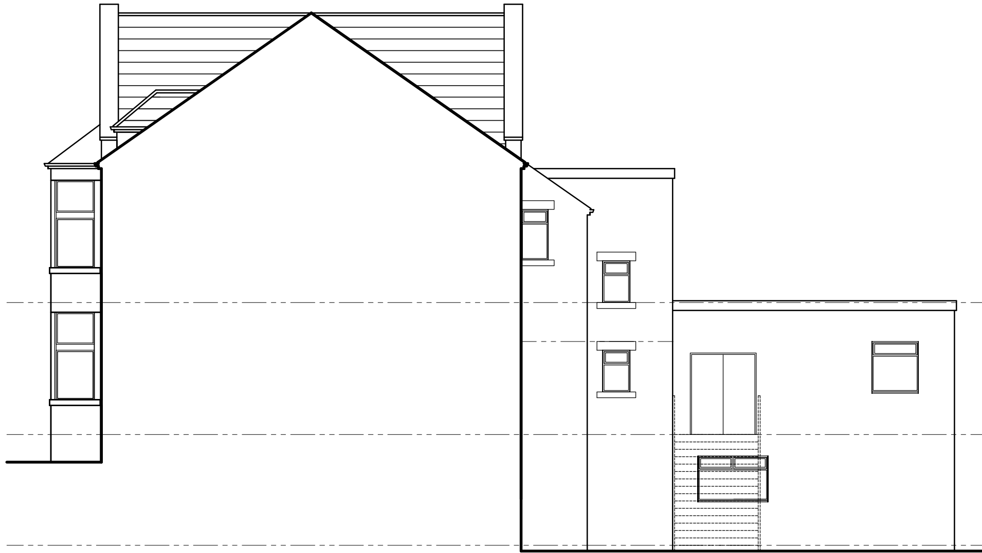
SIDE ELEVATION
