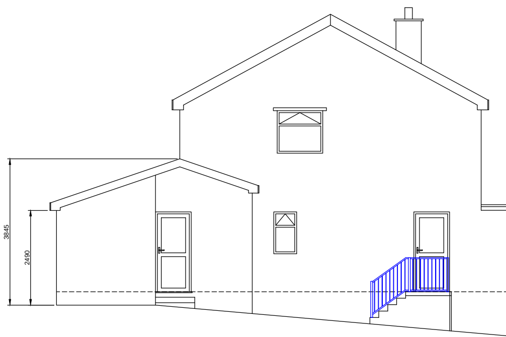
LHS ELEVATION (From No 52)
