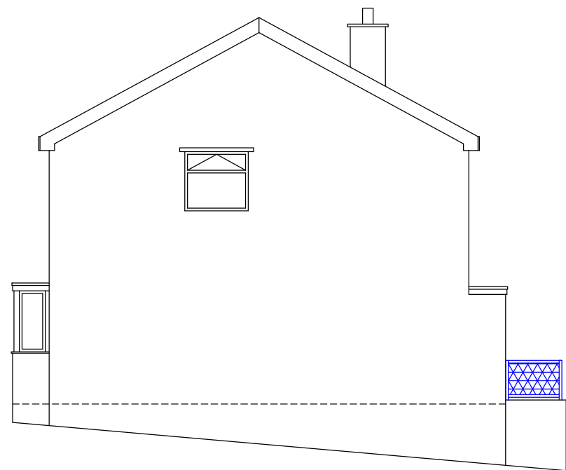
LHS ELEVATION (From No 52)
