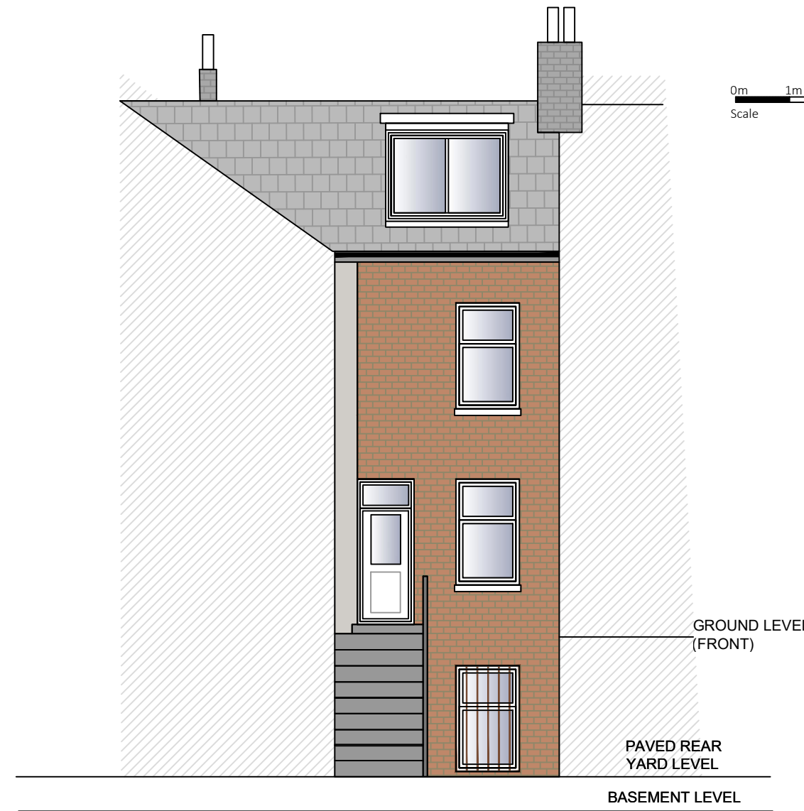
REAR VIEW
