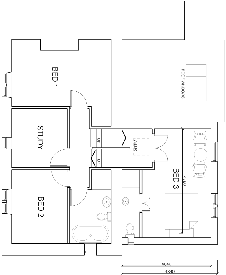
FIRST FLOOR LAYOUT AS PROPOSED
