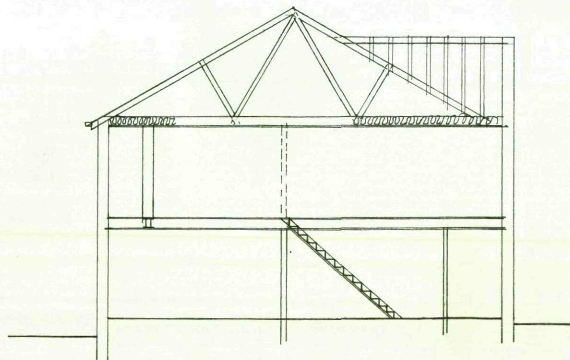
Typical Section
