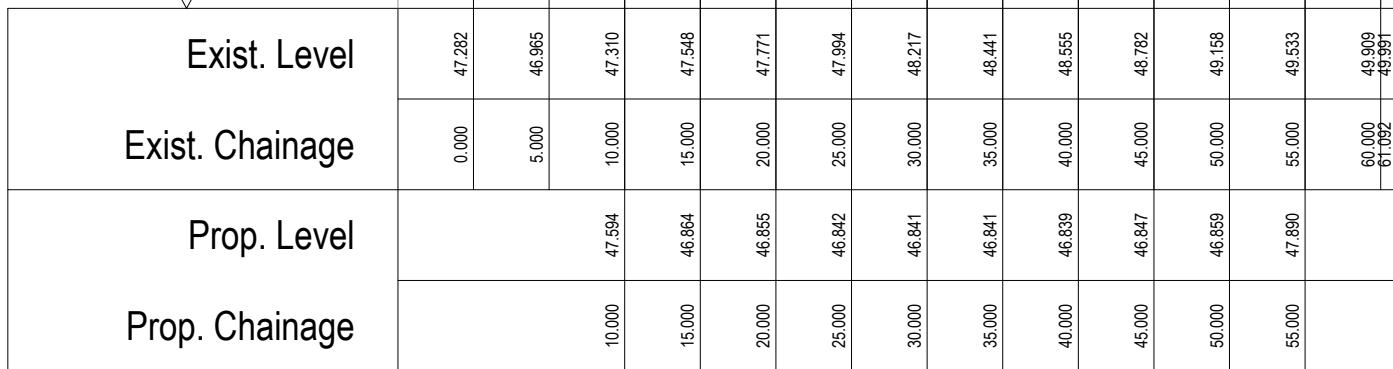
BASIN B-B Horiz. 1:500 Vert. 1:100 44.00 A.O.D.
