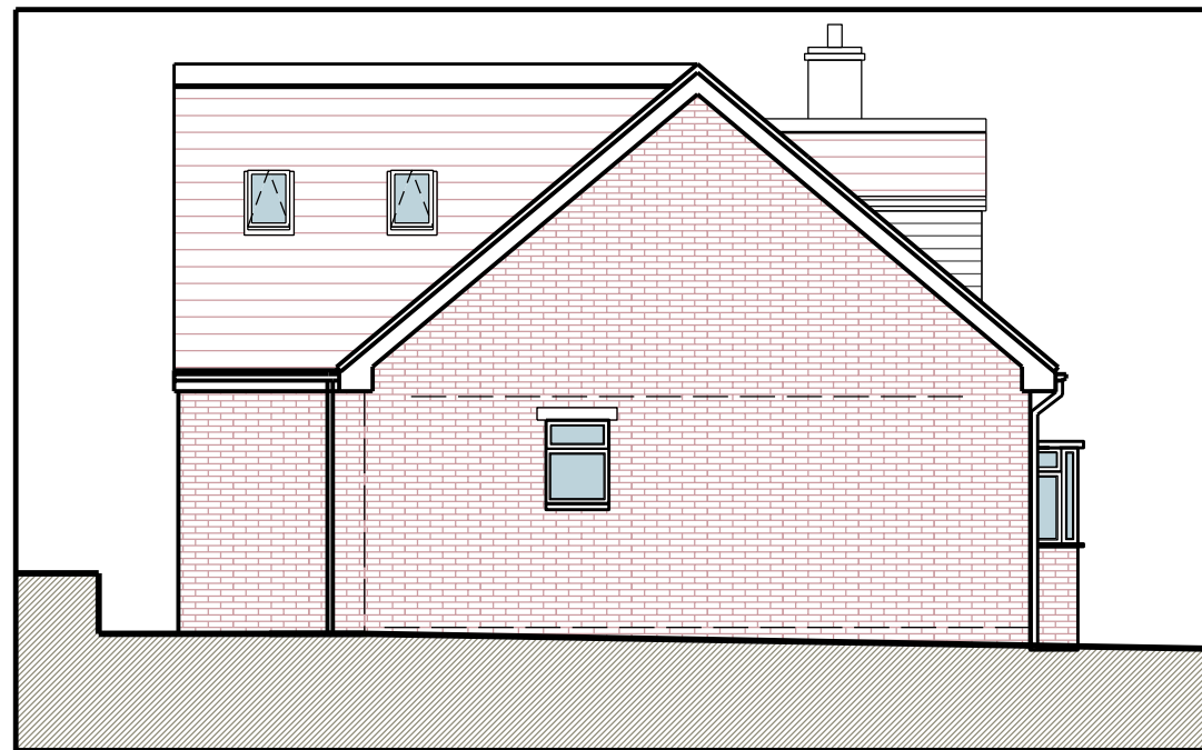
South Elevation
