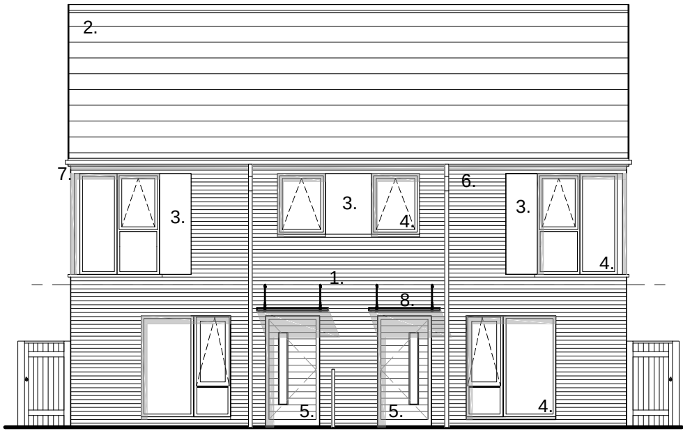
Front Elevation
