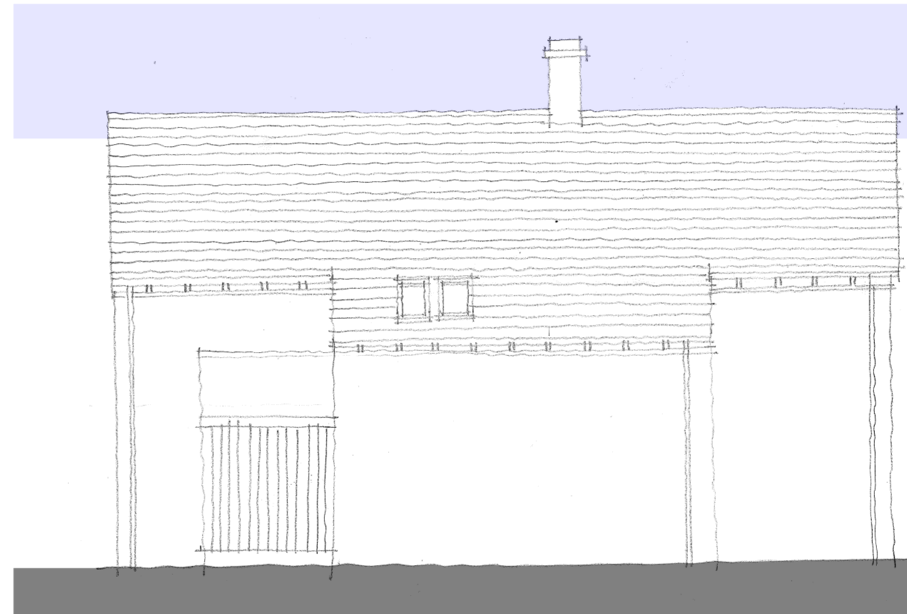
SOUTH ELEVATION
