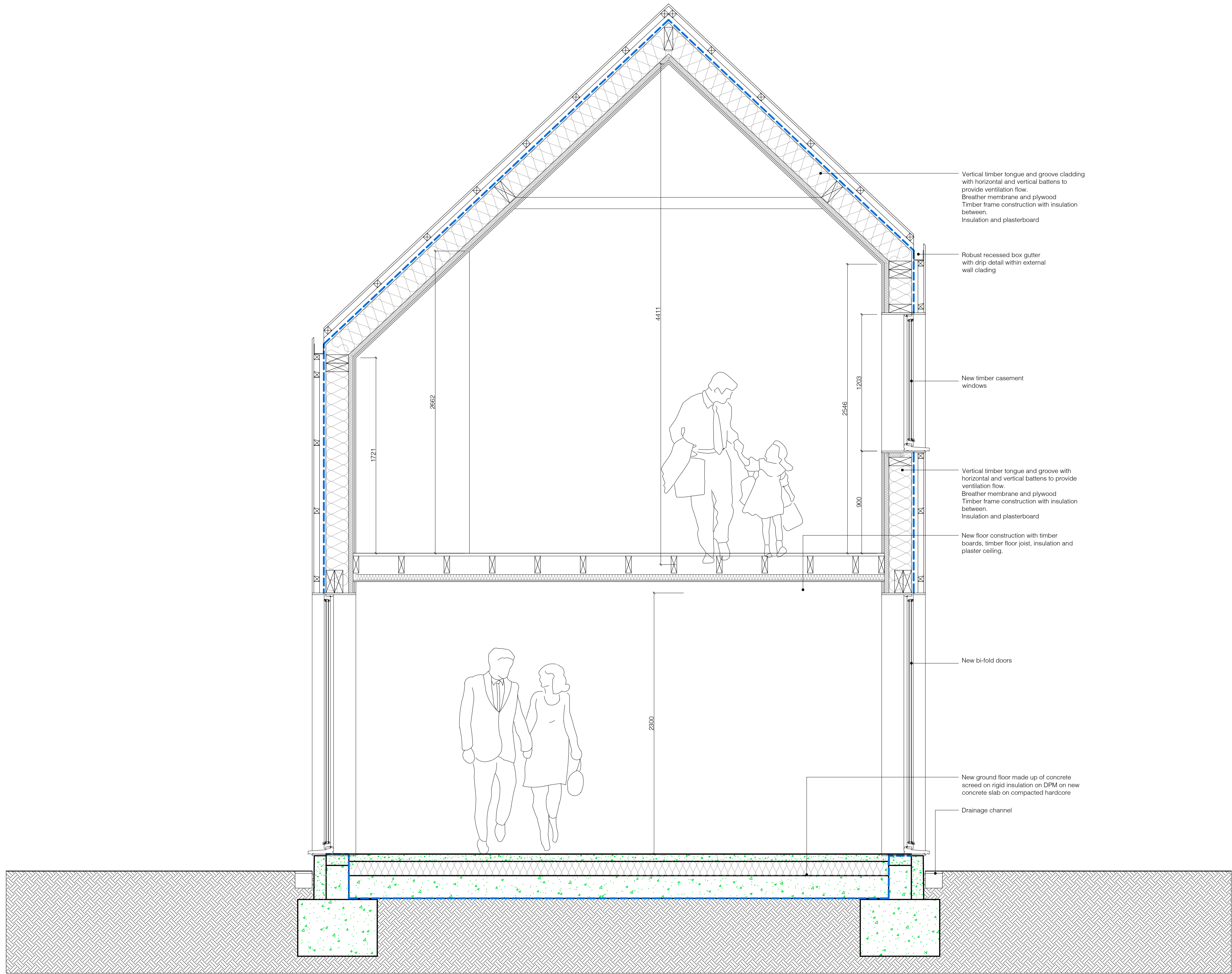
New Dwelling Proposed section AA
